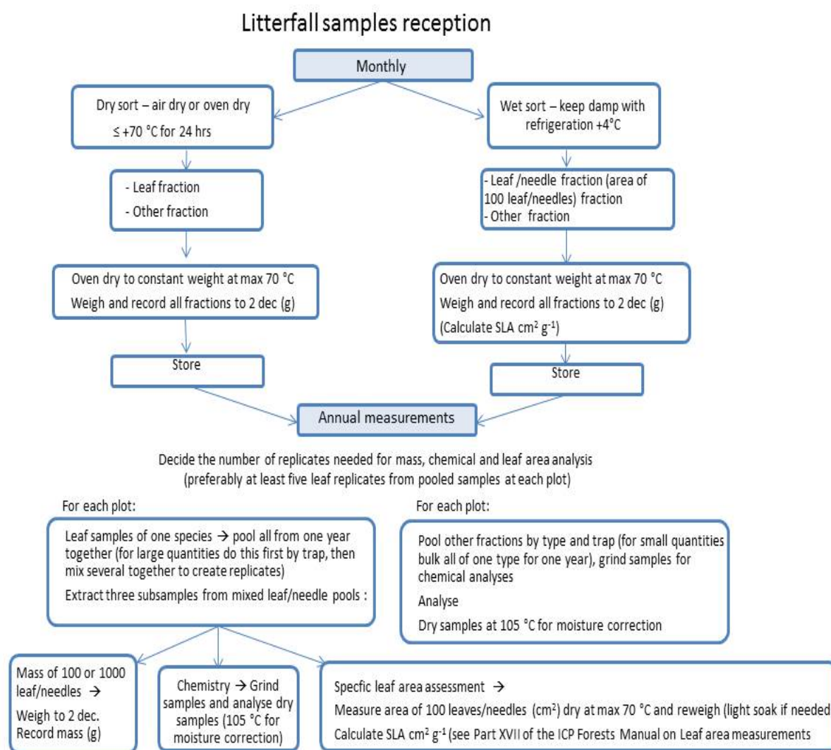
Figure 2: Procedural flow diagram for pretreatment of litter samples
